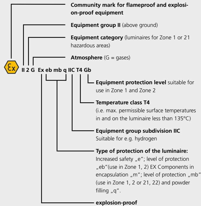
Figure 8: Example of marking of an explosion-protected luminaire
